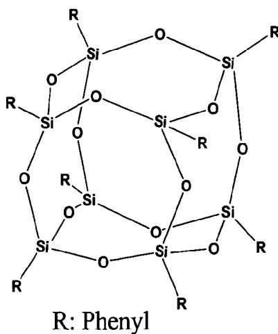
octaphenyl-polyhedral oligomeric silsesquioxane
