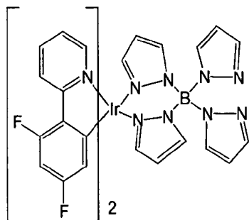
\text{Ir}(4,6\text{-F}_2\text{ppy})_2(\text{BPz}_4)
