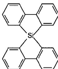
5,5'-Spiro(dibenzosilole)
