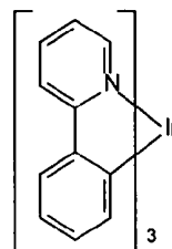
\text{Irppy}
