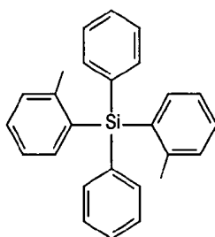
\text{Siph}_2(\text{o-tolyl})_2
